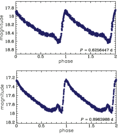
Typical light curves of anomalous Cepheids pulsating in the fundamental mode: OGLE-LMC-ACEP-068 (top), OGLE-LMC-ACEP-007 (bottom). Soszyński et al. (2008) - http://ogle.astrouw.edu.pl
