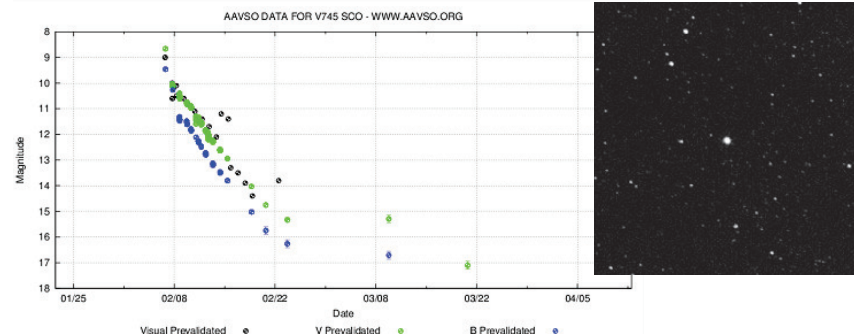
V745 Scorpii photometric observations between 2/6/2014 and 3/22/2014. The chart is generated by the AAVSO web service. The nova outburst was detected on February 6, 2014 by Rod Stubbings from Australia during an early morning observing session. The first CCD image was taken by Steve O' Connor (Bermuda)
