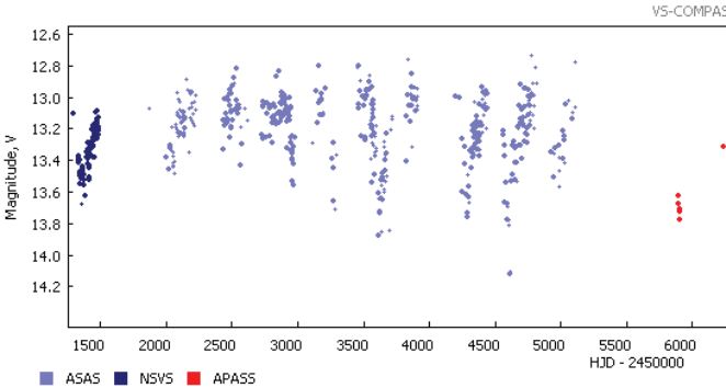
Figure 2. - The light curve of NSV 13538, built of the combined photometric data from the ASAS-3, NSVS and the APASS surveys.
