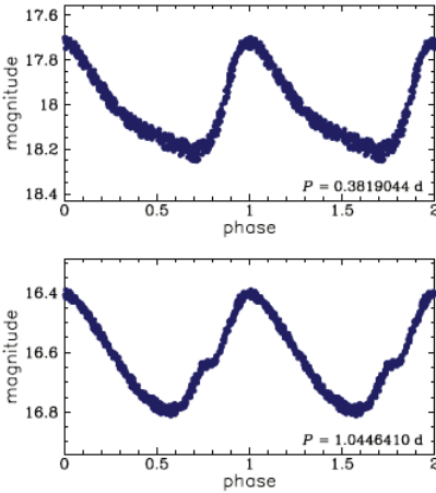
Typical light curves of the first-overtone anomalous Cepheids pulsating: OGLE-LMC-ACEP-020 (top), OGLE-LMC-ACEP-050 (bottom). Soszyński et al. (2008) - http://ogle.astrouw.edu.pl
