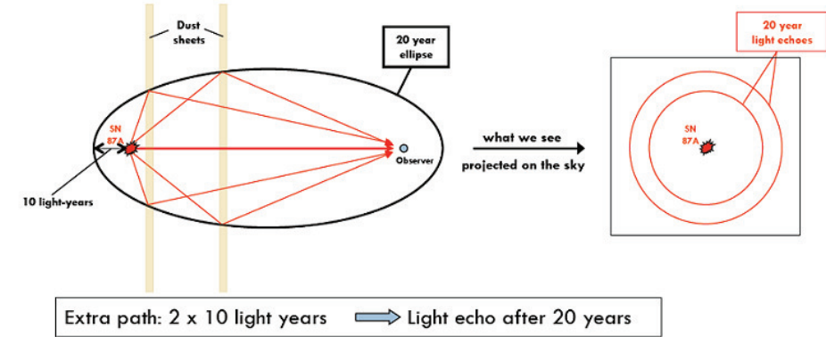
Basic geometry behind a light echo: ellipsoids trace out surfaces of constant arrival time, causing an observer to see distant dust regions being highlighted by the exploded star as concentrated circles projected on the sky. Image credit: Armin Rest (Harvard), SuperMACHO & EHS collaboration
