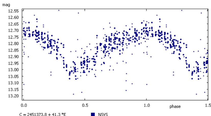
2MASS J18144389+5531238 with the period of 41.3 days shows a typical "flat-topped" curve. by Ivan Sergey, Andrey Prokopovich (VS-COMPAS)
