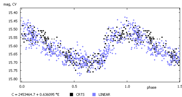
CSS J130739.5+011029 in Virgo by Andrey Prokopovich, Ivan Adamin (VS-COMPAS) J-K = 0.2. Secondary period is 0.62179
