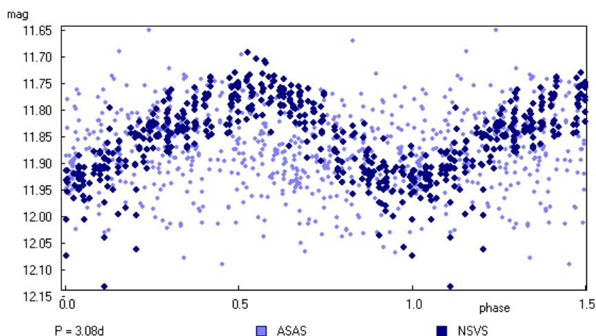
2MASS J05003003+1723591 (WTTS/ROT). Period is 3.08 days. by Andrey Prokopovich, Ivan Adamin (VS-COMPAS), Sebastian Otero
