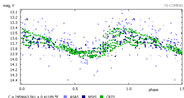
NSVS 10564788 in Bootes by Alexandr Ditzkovsky (VS-COMPAS) J-K= 0.214
