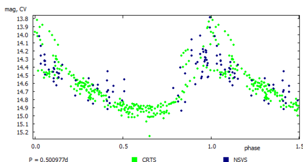
VSX J133154.0+300010 in Canes Venatici by Alexandr Ditzkovsky (VS-COMPAS)
