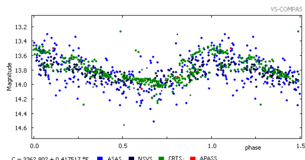
NSVS 10303225 in Leo by Alexandr Ditzkovsky (VS-COMPAS) NSVS and ASAS-3 data are contaminated by 2MASS J10430453+0903402 (V= 14.9, sep. 24"). Data has been debledned. J-K= 0.23
