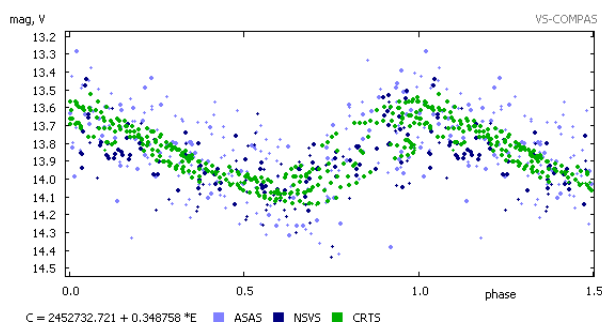
NSVS 13082928 in Leo by Alexandr Ditzkovsky (VS-COMPAS) J-K = 0.238
