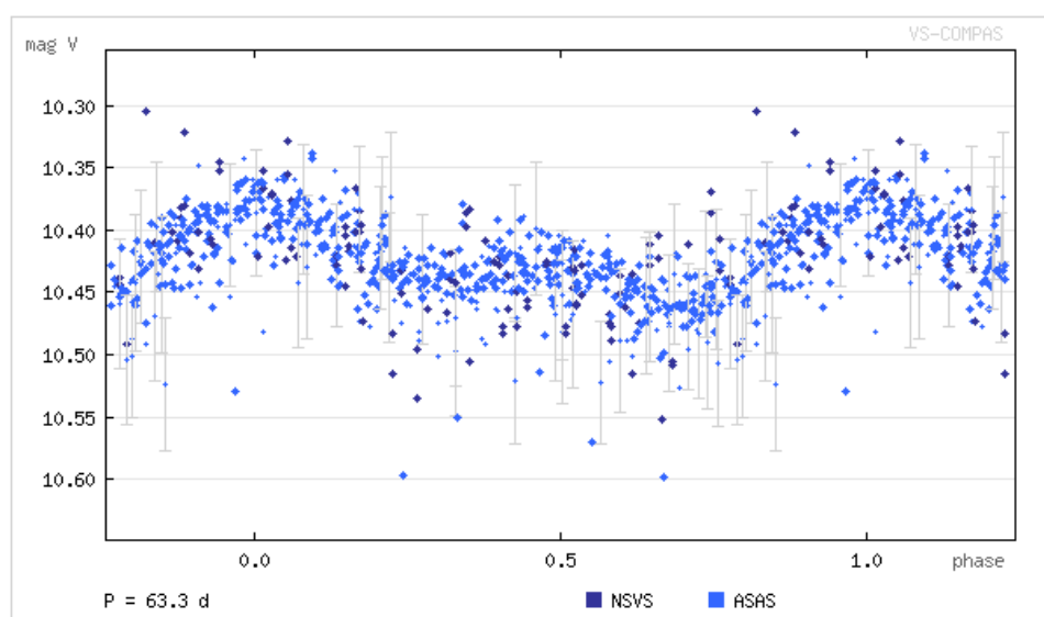
NSVS 15314262. Folded light curve. M = HJD\ 2453077.0 + 63.29 * E . by Alexandr Ditkovsky (VS-COMPAS)
