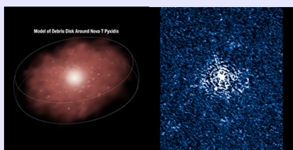
Debris disk around T Pyxidis star
