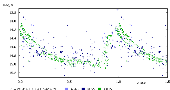
VSX J092806.8+090728 in Leo by Alexandr Ditzkovsky (VS-COMPAS) J-K = 0.23
